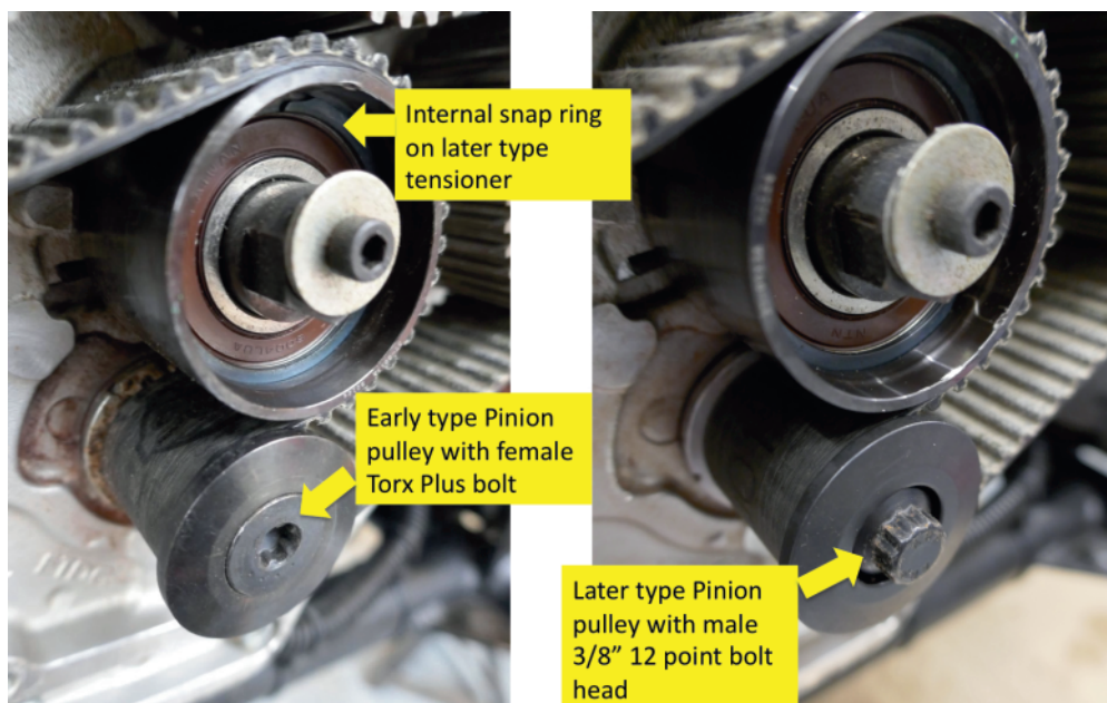
Figure 6 Cam chamber pinion pulley and tensioner detail
